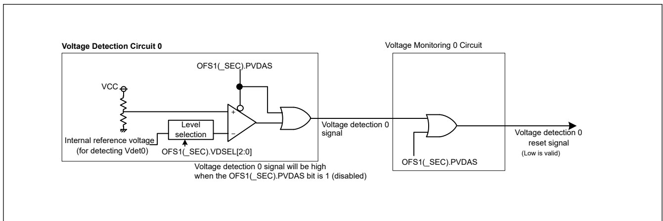
Figure 8.1 Block diagram of voltage monitor 0 reset circuit
